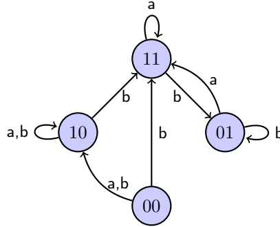
Figure 2: Example model of accessibility relations among outlooks
