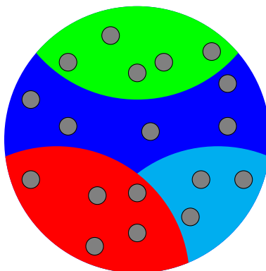
Figure 1: Possible worlds (shaded areas) and the outlooks that refine them
